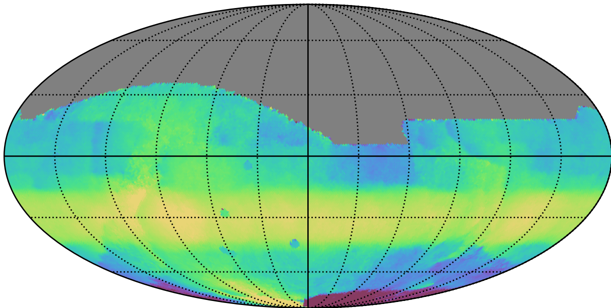
no_magell_roll_v3.4_10yrs All sky all bands: Median HA
