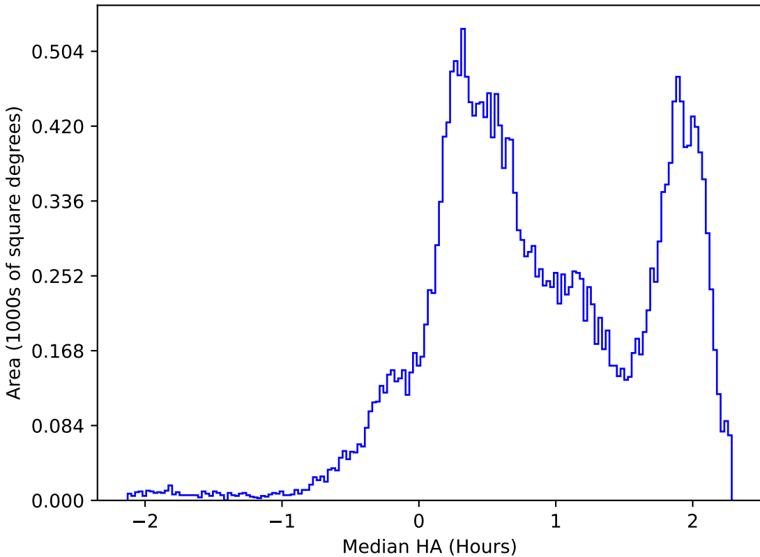
no_magell_roll_v3.4_10yrs All sky all bands: Median HA
