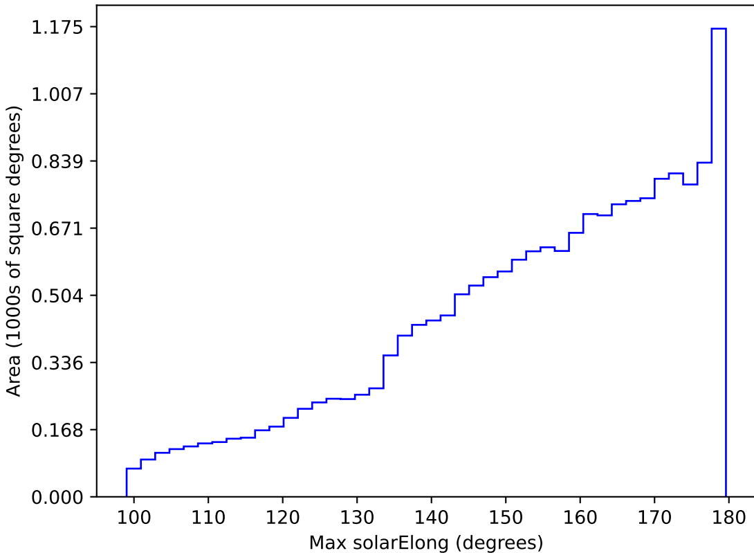
no_magell_roll_v3.4_10yrs WFD all bands: Max solarElong
