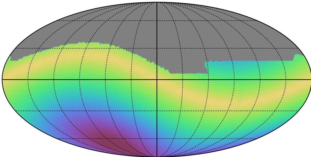
no_magell_roll_v3.4_10yrs All sky all bands: Max solarElong
