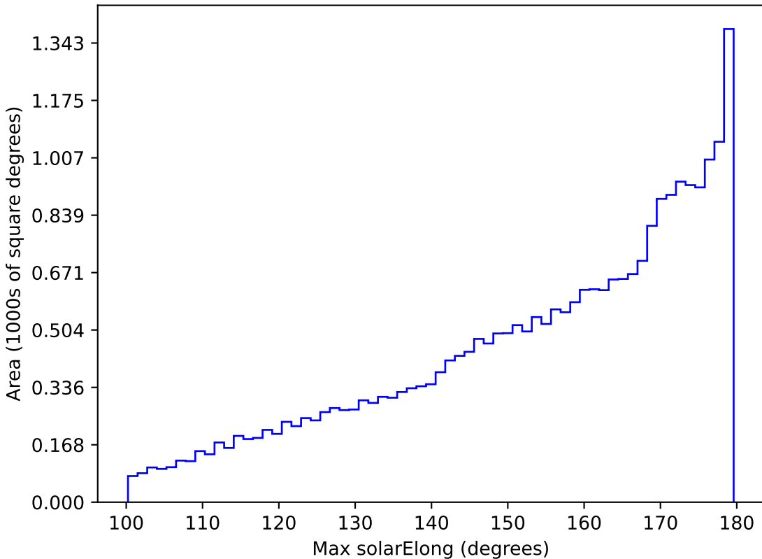
no_magell_roll_v3.4_10yrs All sky all bands: Max solarElong
