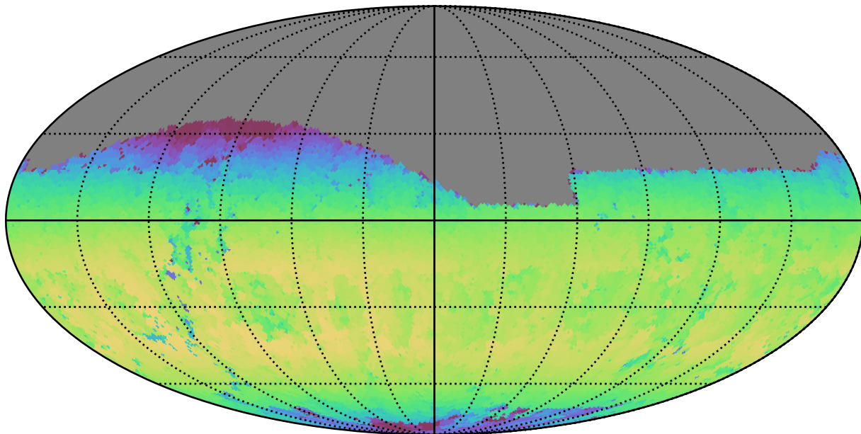
no_magell_roll_v3.4_10yrs Yr 1 z band: Max skyBrightness
