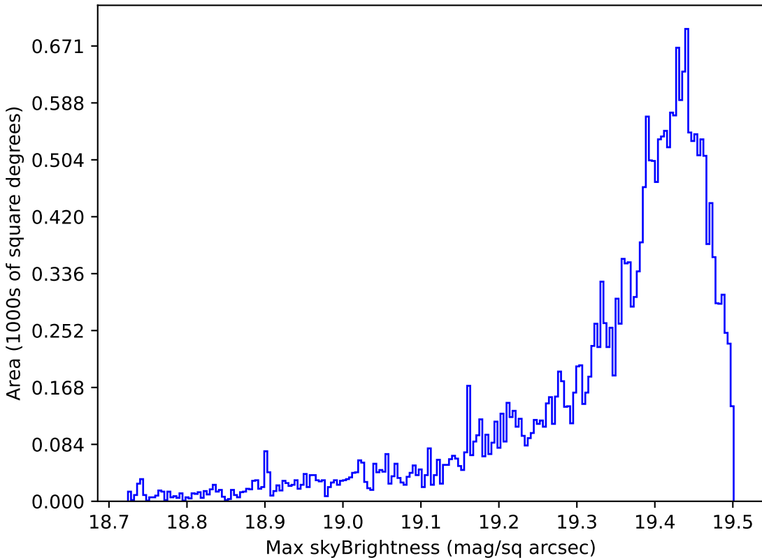
no_magell_roll_v3.4_10yrs Yr 1 z band: Max skyBrightness
