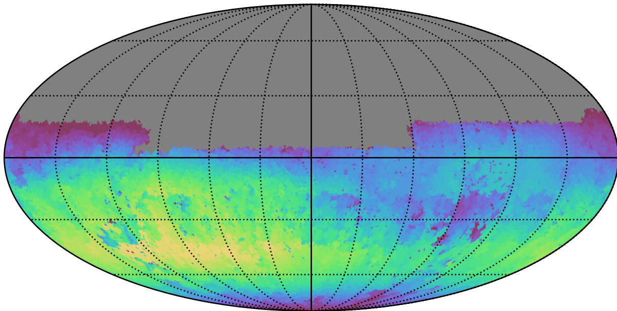
no_magell_roll_v3.4_10yrs Yr 1 u band: Max skyBrightness
