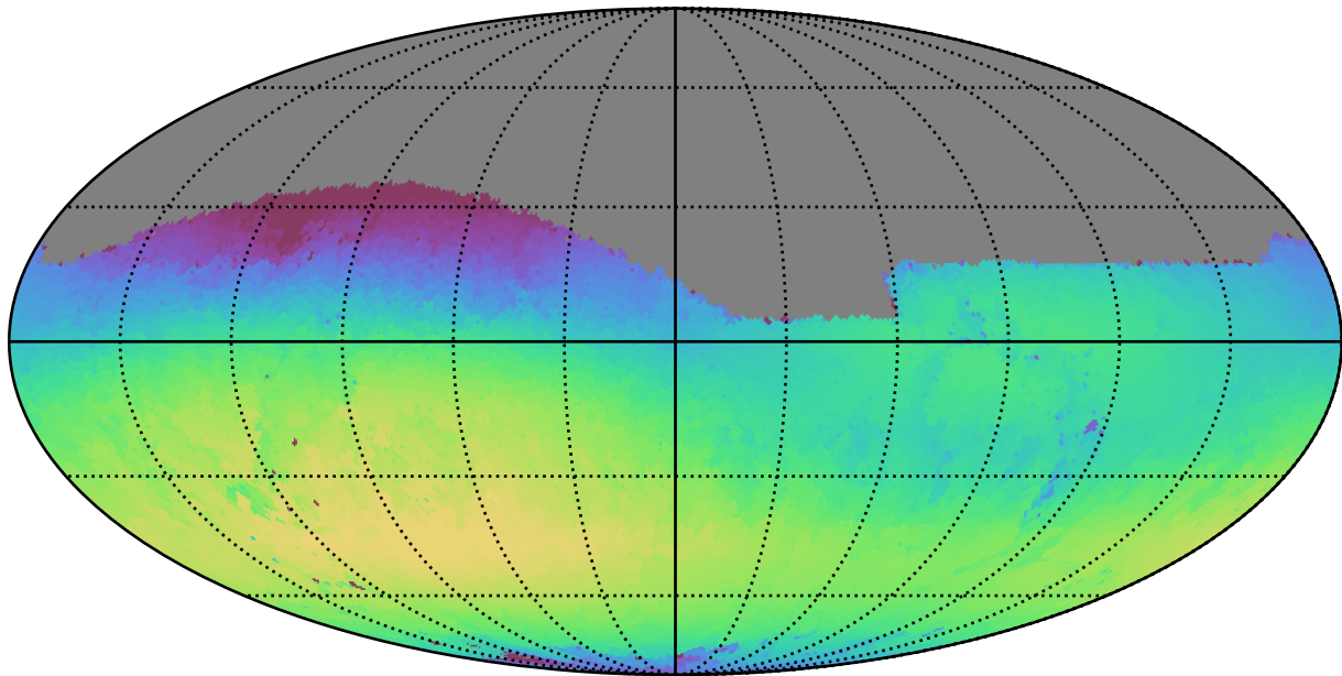
no_magell_roll_v3.4_10yrs Yr 1 r band: Max skyBrightness
