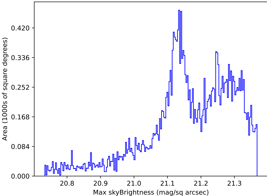
no_magell_roll_v3.4_10yrs Yr 1 r band: Max skyBrightness
