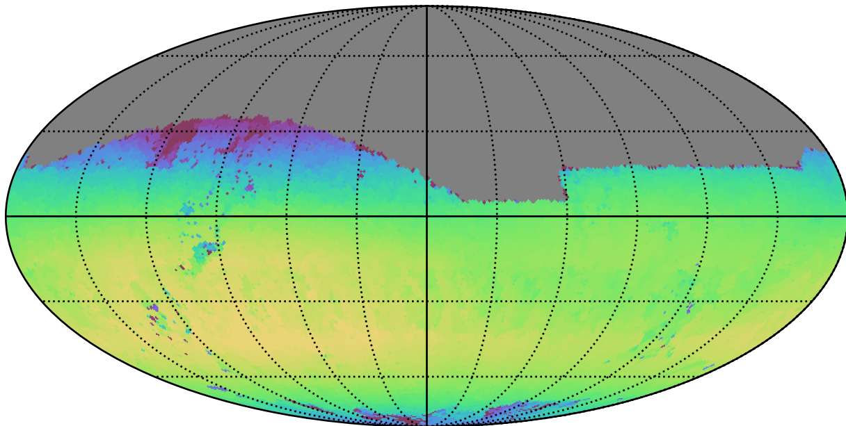
no_magell_roll_v3.4_10yrs Yr 1 i band: Max skyBrightness
