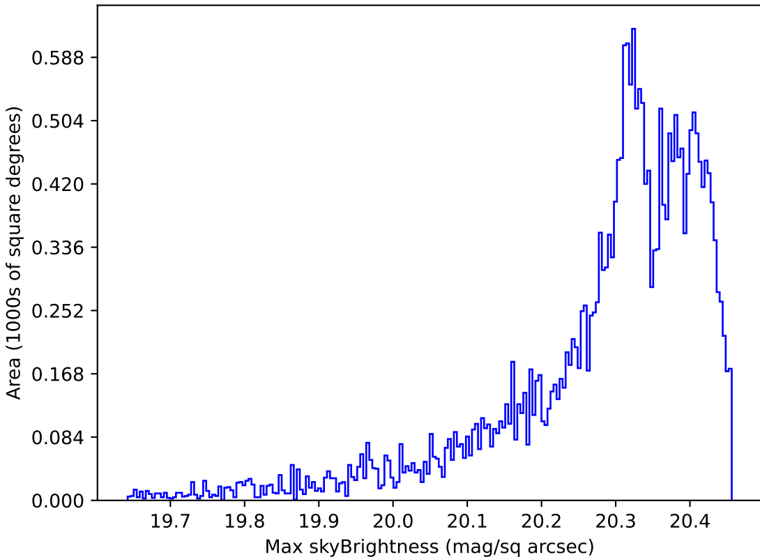
no_magell_roll_v3.4_10yrs Yr 1 i band: Max skyBrightness
