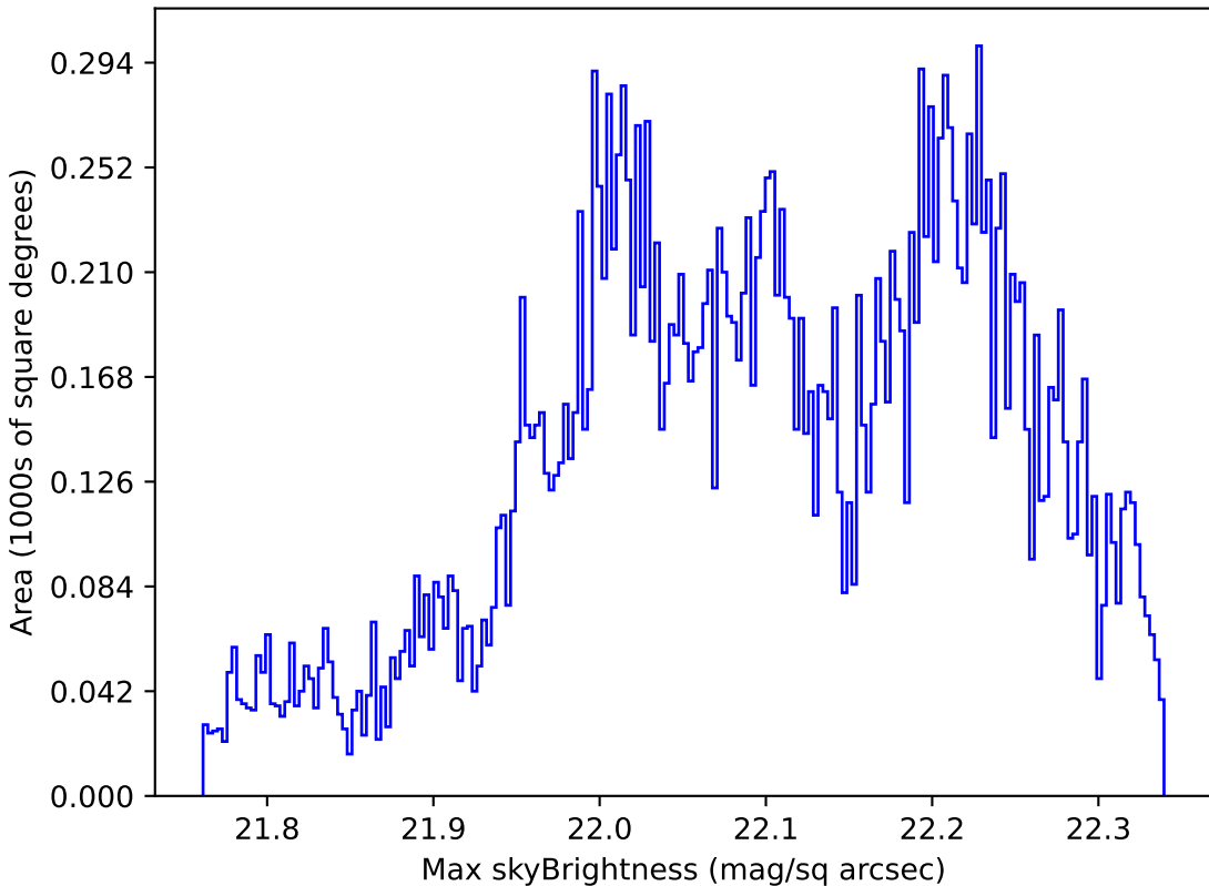
no_magell_roll_v3.4_10yrs Yr 1 g band: Max skyBrightness
