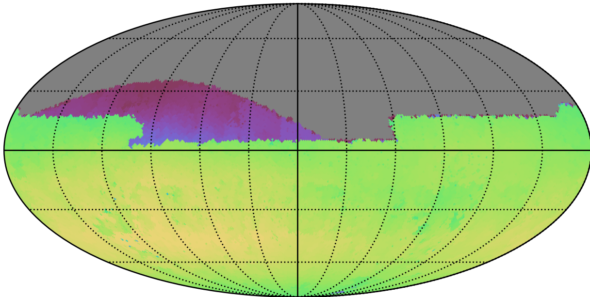
no_magell_roll_v3.4_10yrs Yr 1 all bands: Max skyBrightness
