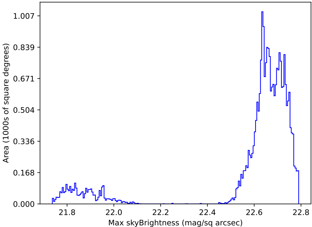
no_magell_roll_v3.4_10yrs Yr 1 all bands: Max skyBrightness
