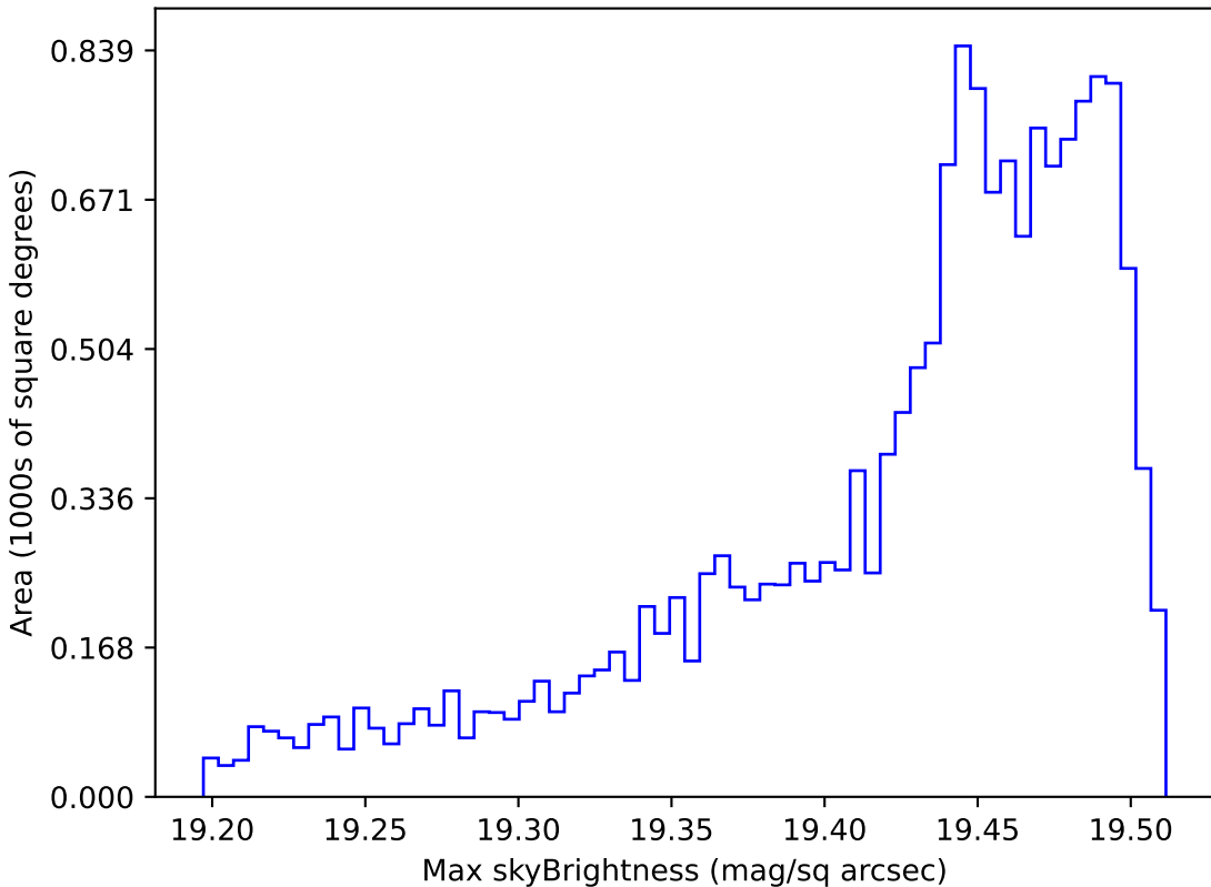
no_magell_roll_v3.4_10yrs WFD z band: Max skyBrightness
