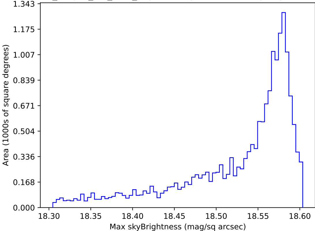
no_magell_roll_v3.4_10yrs WFD y band: Max skyBrightness
