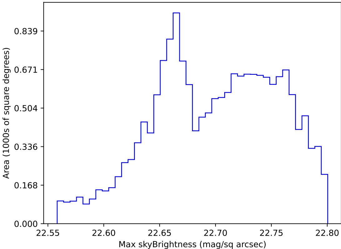
no_magell_roll_v3.4_10yrs WFD u band: Max skyBrightness
