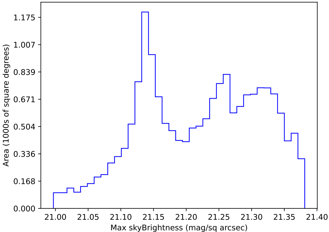
no_magell_roll_v3.4_10yrs WFD r band: Max skyBrightness
