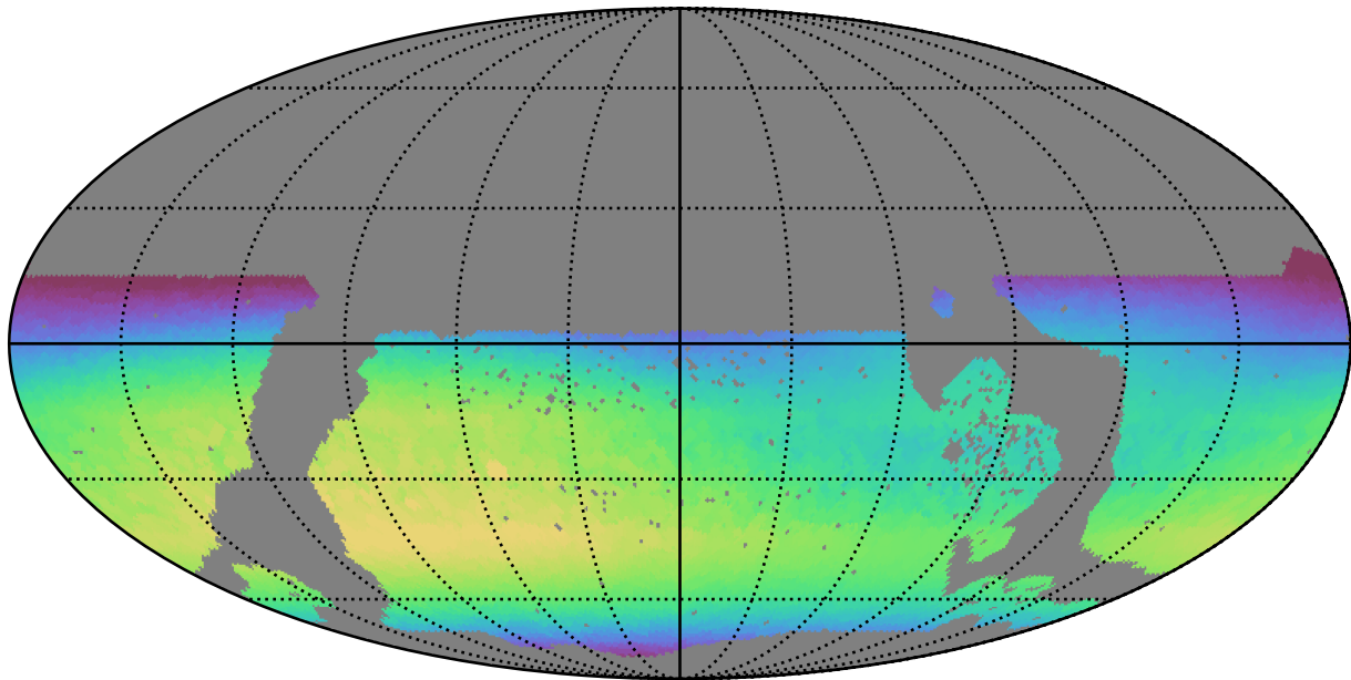
no_magell_roll_v3.4_10yrs WFD i band: Max skyBrightness
