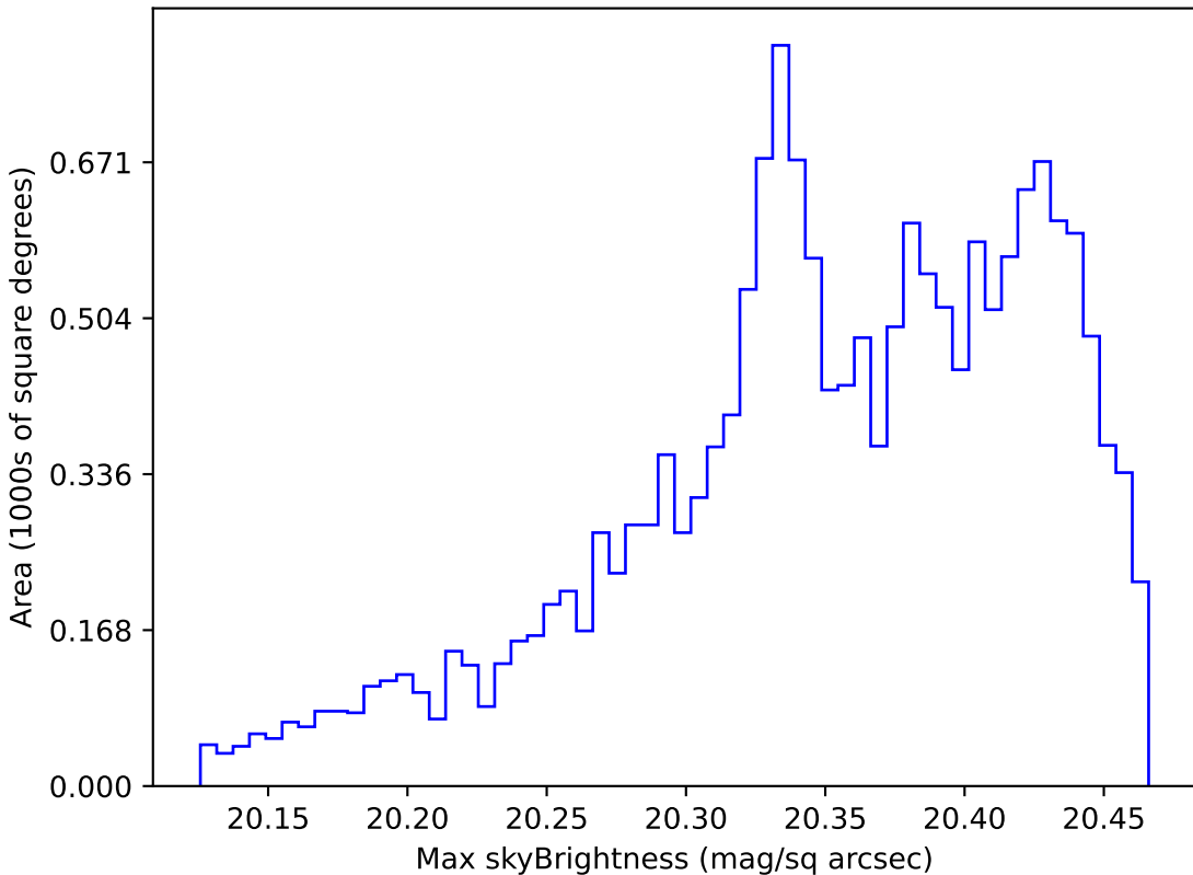
no_magell_roll_v3.4_10yrs WFD i band: Max skyBrightness
