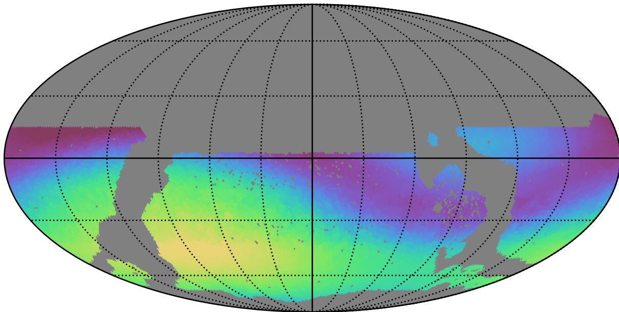
no_magell_roll_v3.4_10yrs WFD g band: Max skyBrightness
