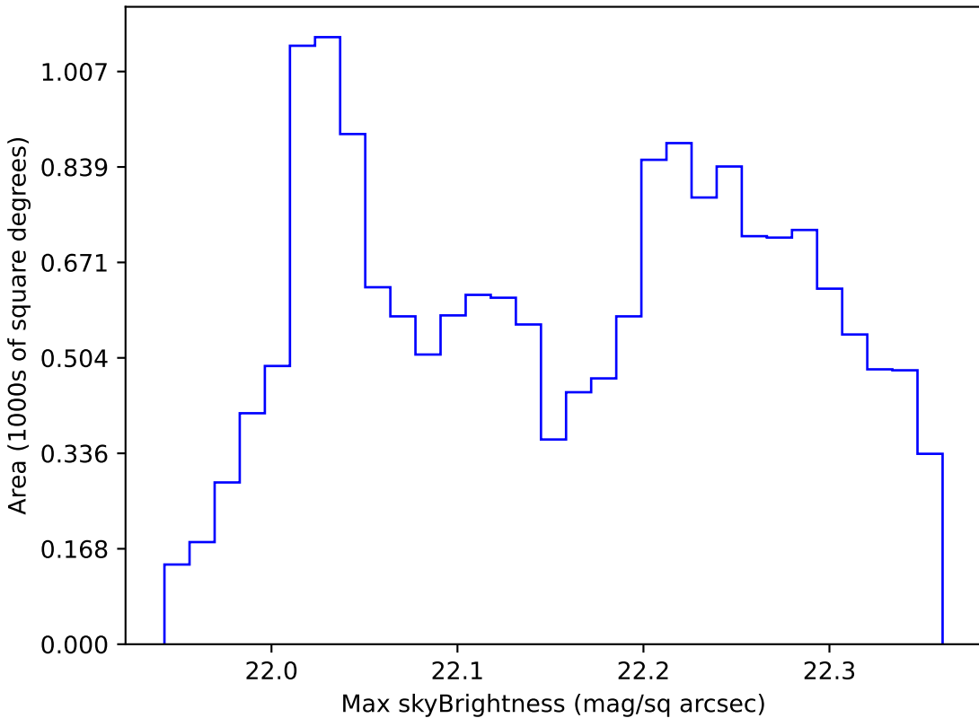
no_magell_roll_v3.4_10yrs WFD g band: Max skyBrightness
