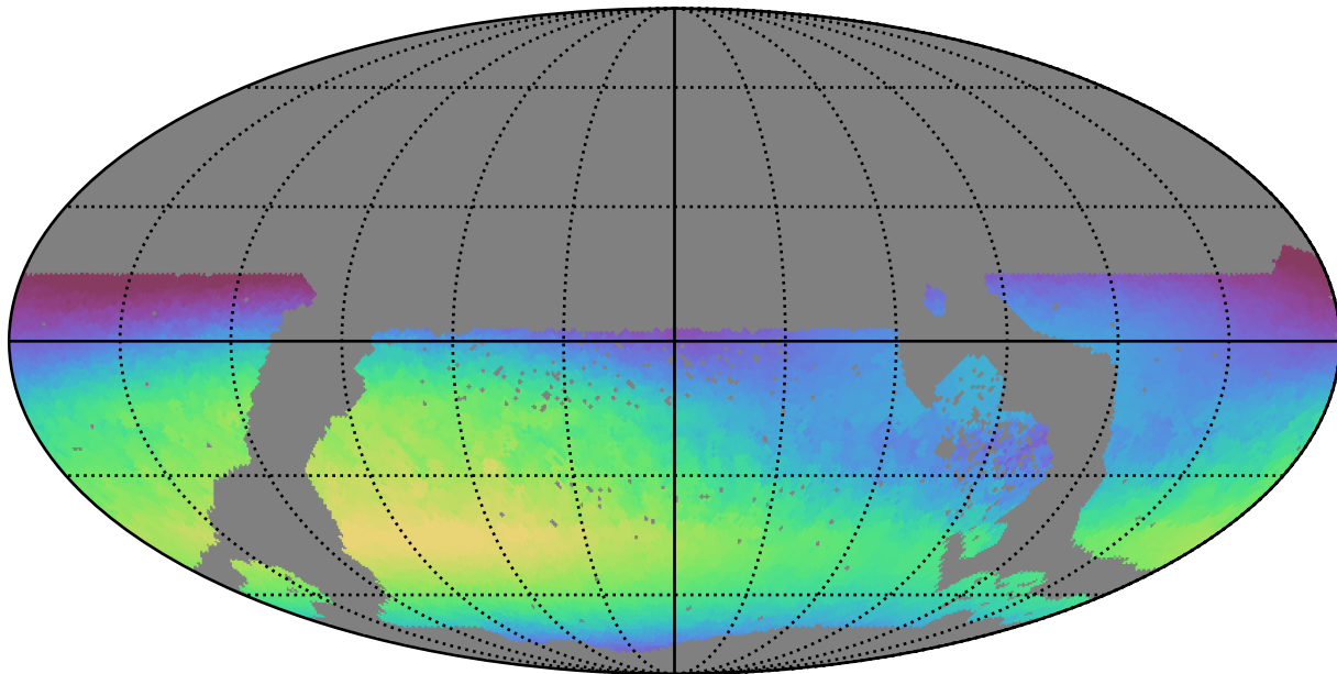
no_magell_roll_v3.4_10yrs WFD all bands: Max skyBrightness
