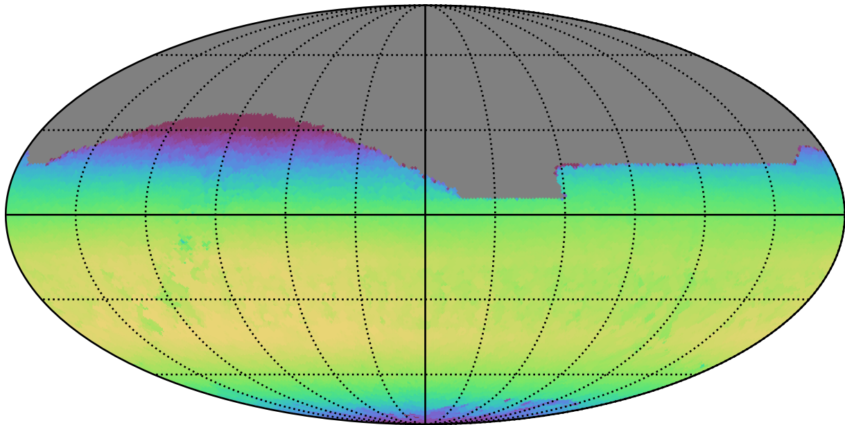
no_magell_roll_v3.4_10yrs All sky z band: Max skyBrightness
