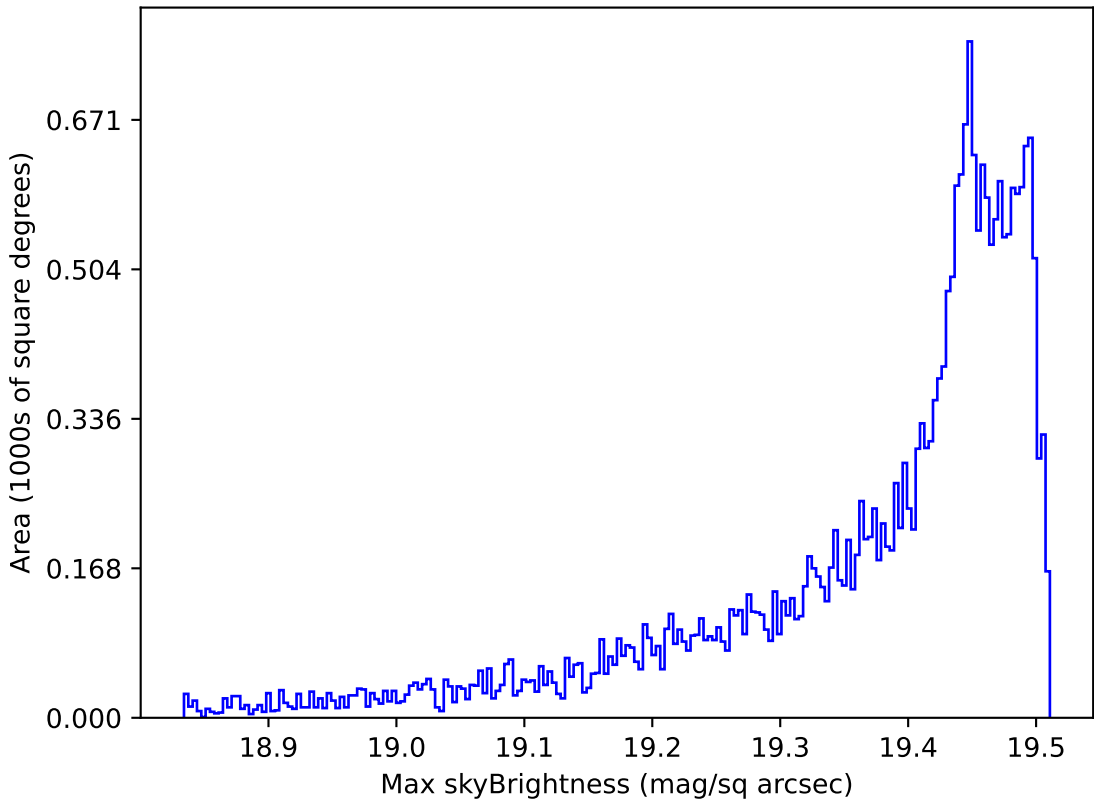
no_magell_roll_v3.4_10yrs All sky z band: Max skyBrightness
