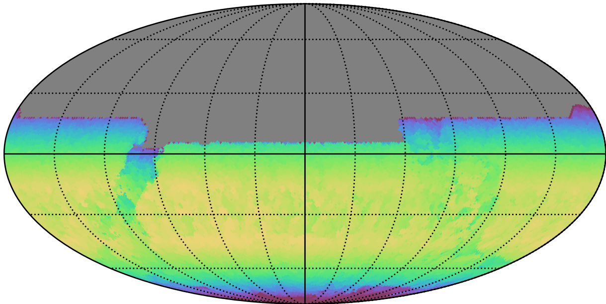
no_magell_roll_v3.4_10yrs All sky y band: Max skyBrightness
