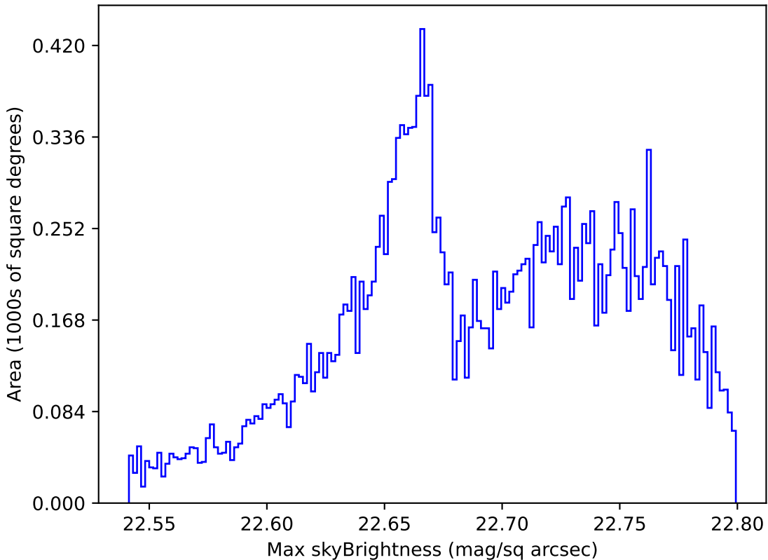
no_magell_roll_v3.4_10yrs All sky u band: Max skyBrightness
