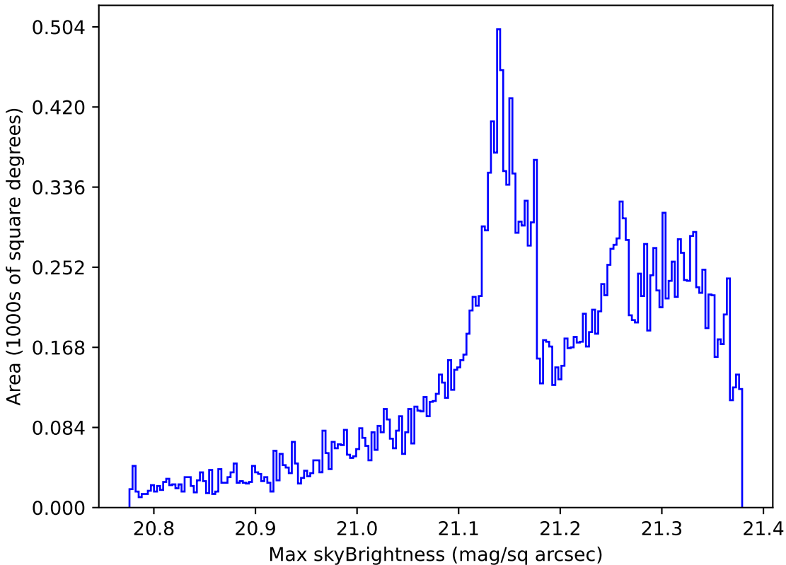
no_magell_roll_v3.4_10yrs All sky r band: Max skyBrightness
