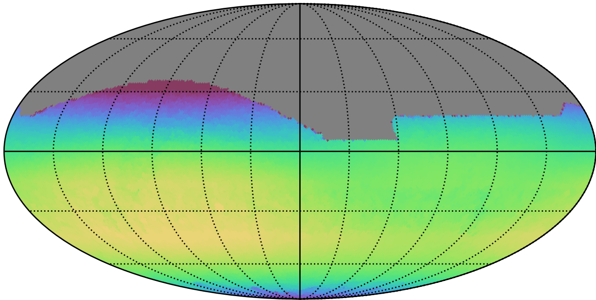
no_magell_roll_v3.4_10yrs All sky i band: Max skyBrightness
