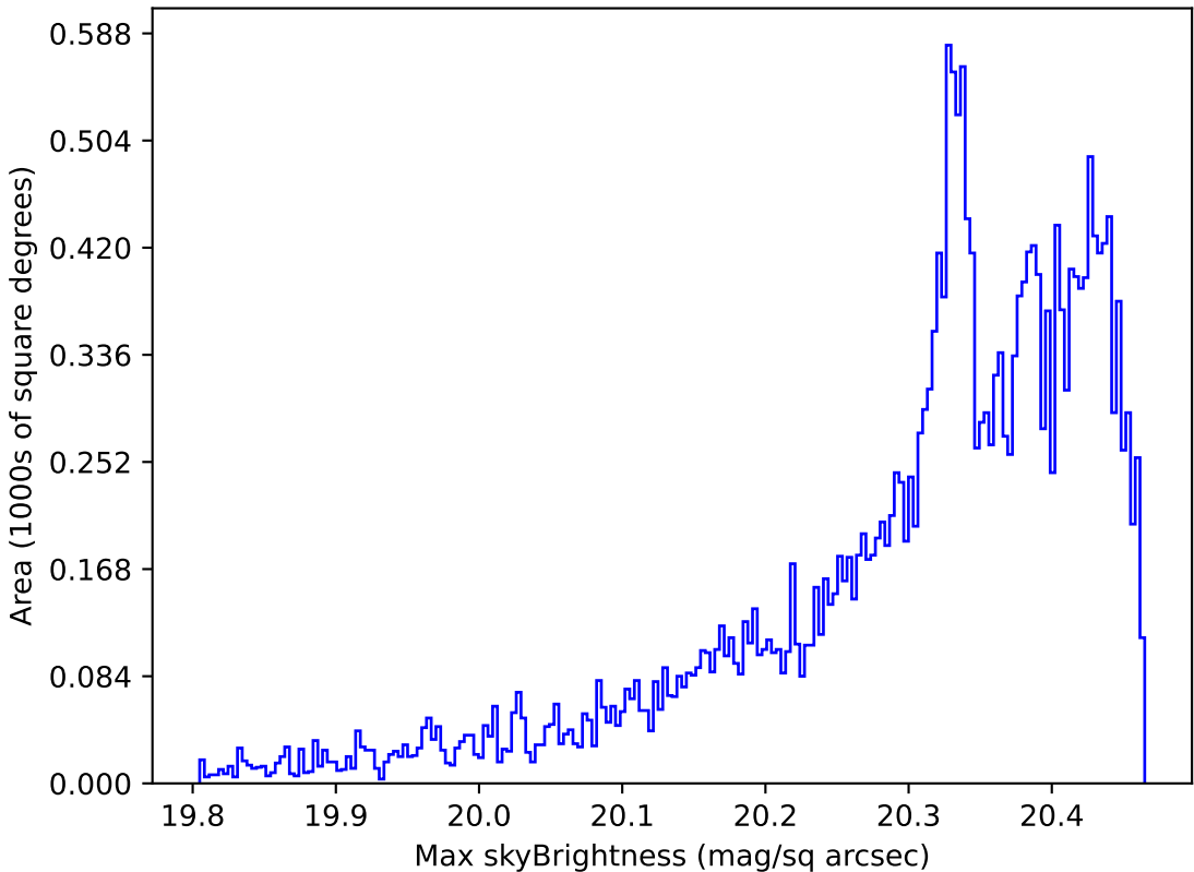
no_magell_roll_v3.4_10yrs All sky i band: Max skyBrightness
