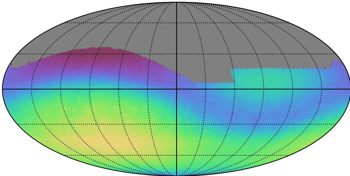
no_magell_roll_v3.4_10yrs All sky g band: Max skyBrightness
