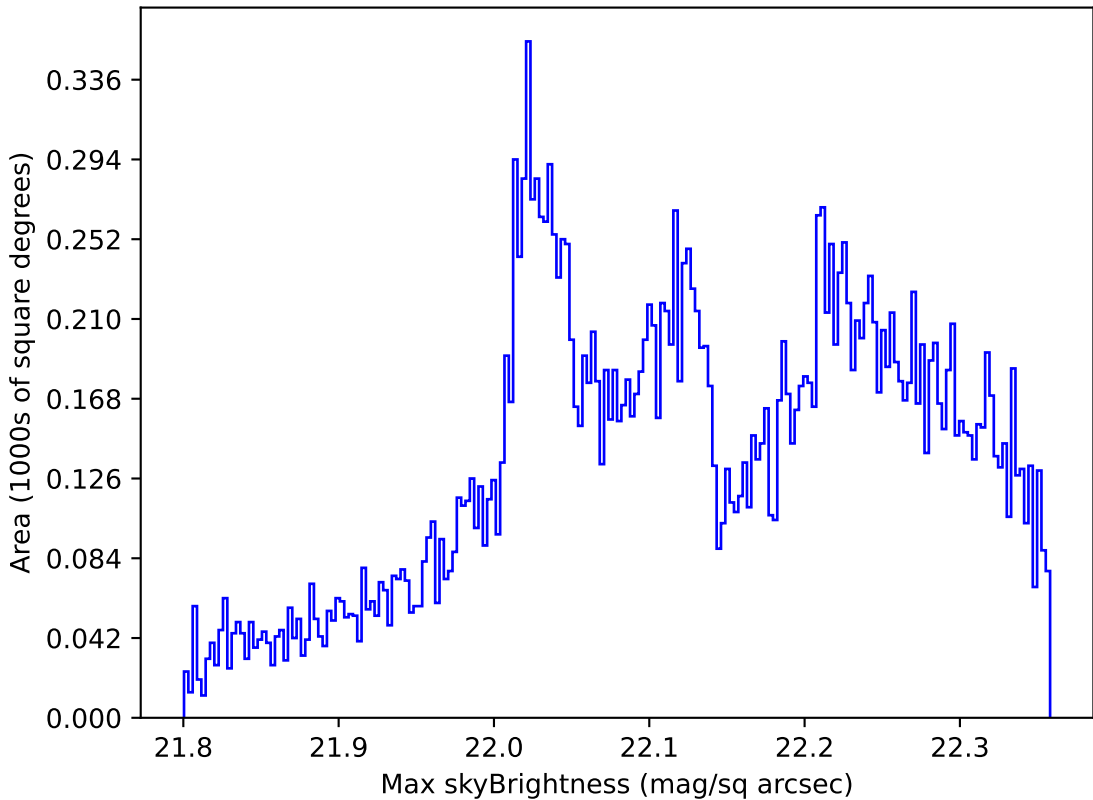
no_magell_roll_v3.4_10yrs All sky g band: Max skyBrightness
