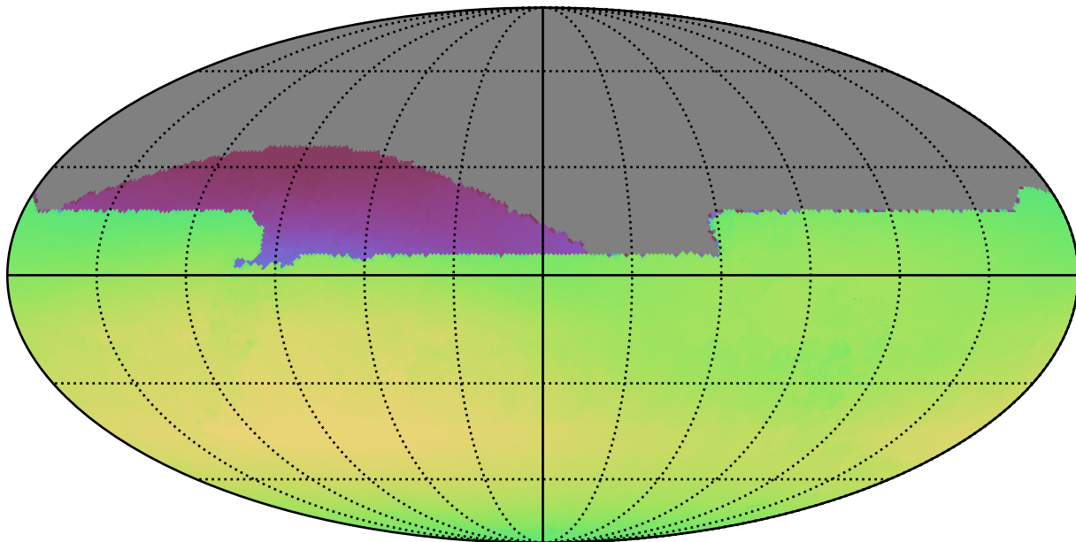
no_magell_roll_v3.4_10yrs All sky all bands: Max skyBrightness
