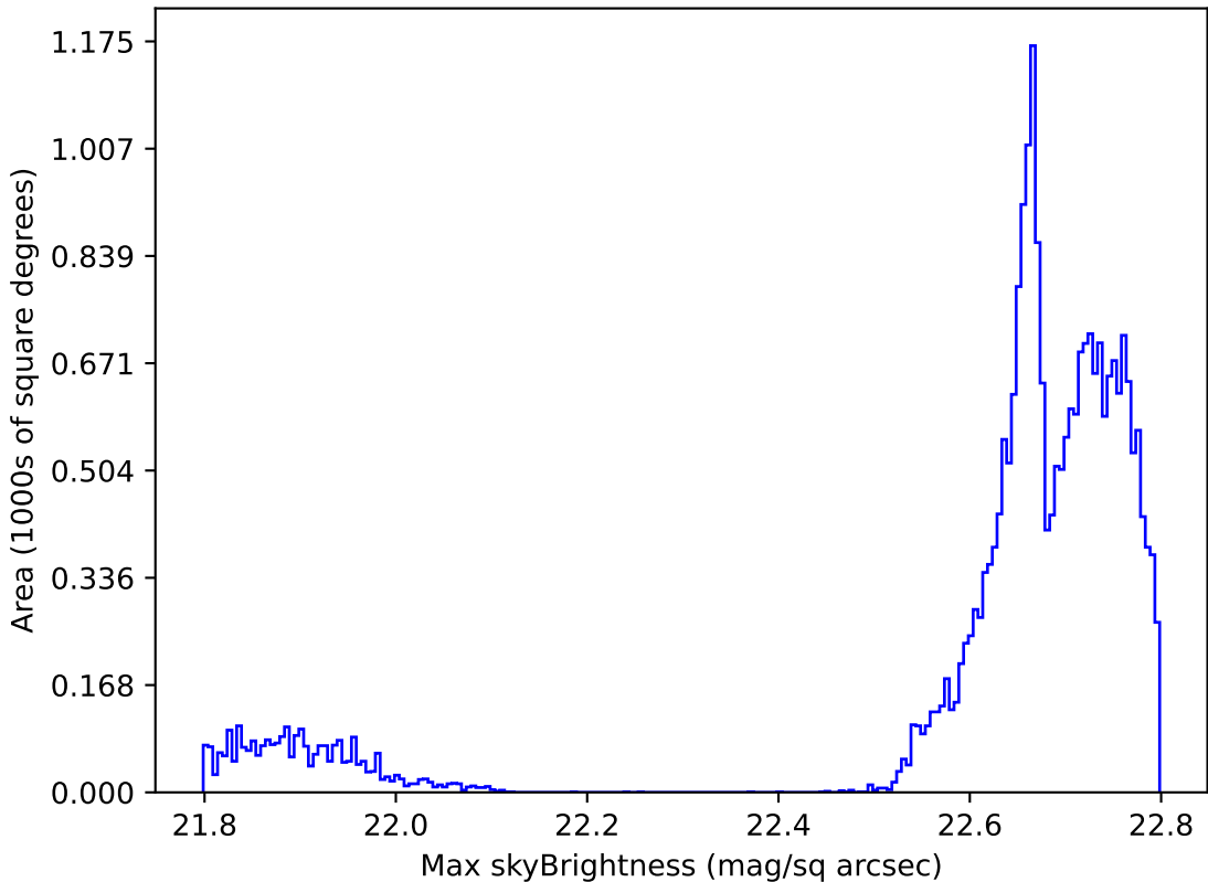
no_magell_roll_v3.4_10yrs All sky all bands: Max skyBrightness
