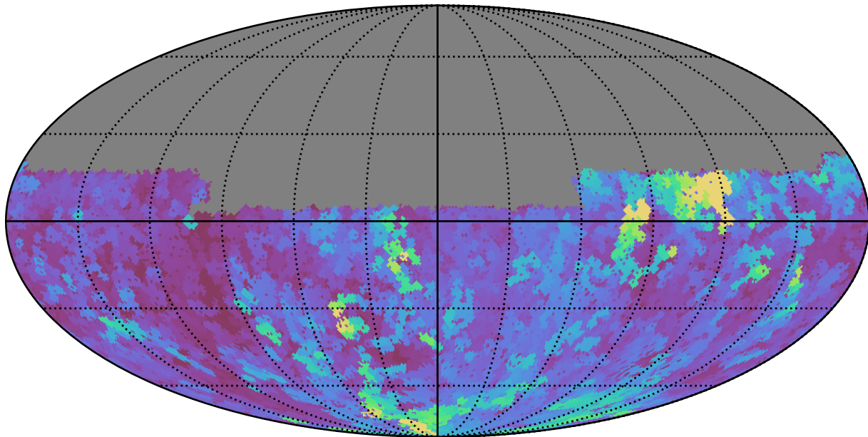
no_magell_roll_v3.4_10yrs Yr 1 u band: Max seeingGeom
