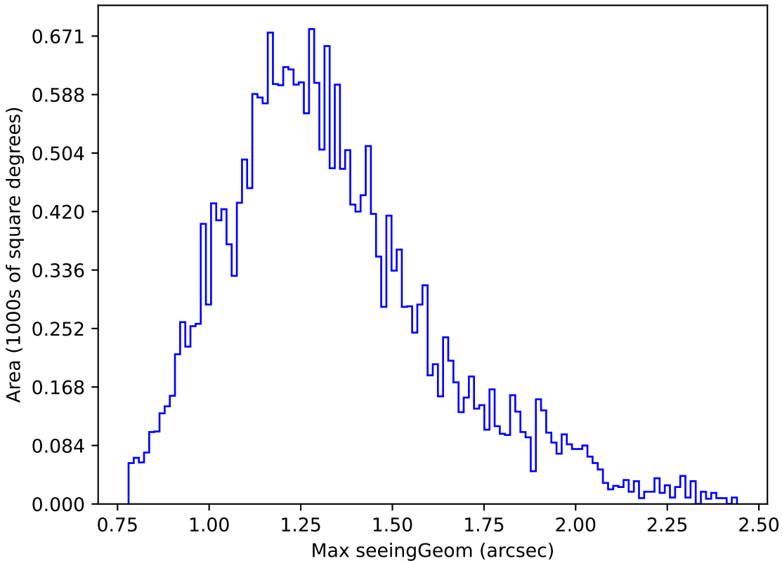
no_magell_roll_v3.4_10yrs Yr 1 r band: Max seeingGeom
