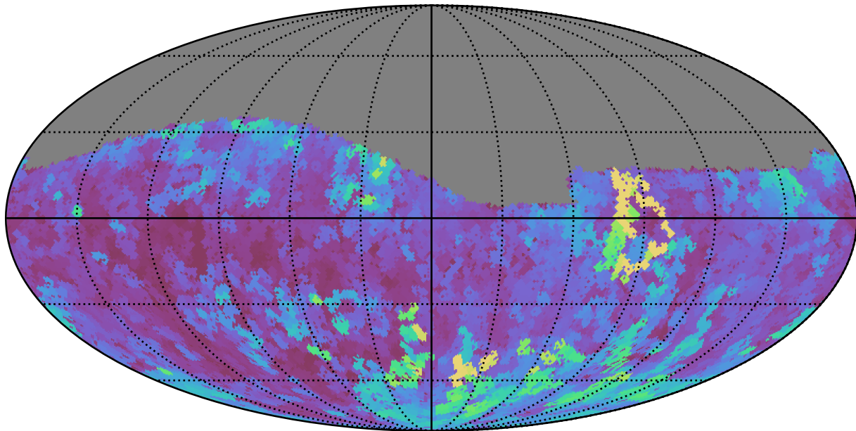
no_magell_roll_v3.4_10yrs Yr 1 g band: Max seeingGeom
