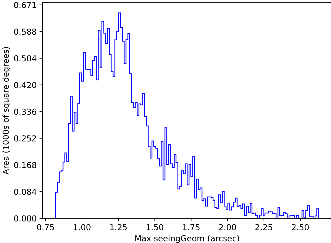
no_magell_roll_v3.4_10yrs Yr 1 g band: Max seeingGeom
