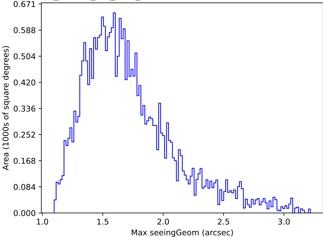
no_magell_roll_v3.4_10yrs Yr 1 all bands: Max seeingGeom
