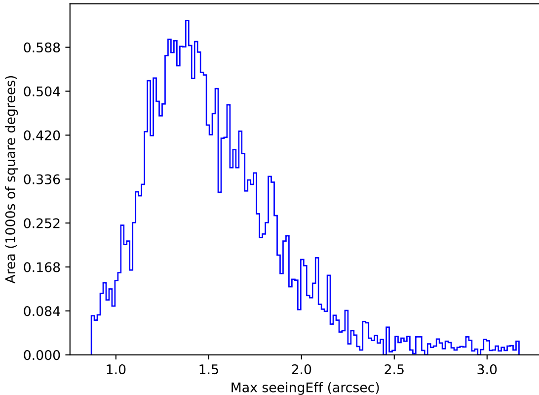
no_magell_roll_v3.4_10yrs Yr 1 z band: Max seeingEff
