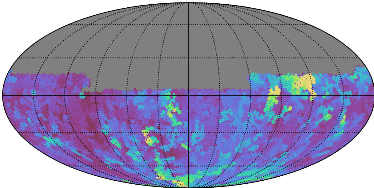
no_magell_roll_v3.4_10yrs Yr 1 u band: Max seeingEff
