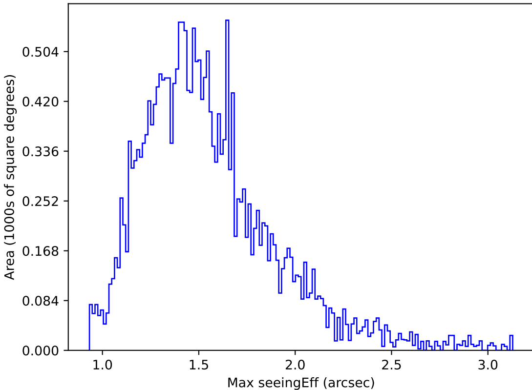
no_magell_roll_v3.4_10yrs Yr 1 u band: Max seeingEff
