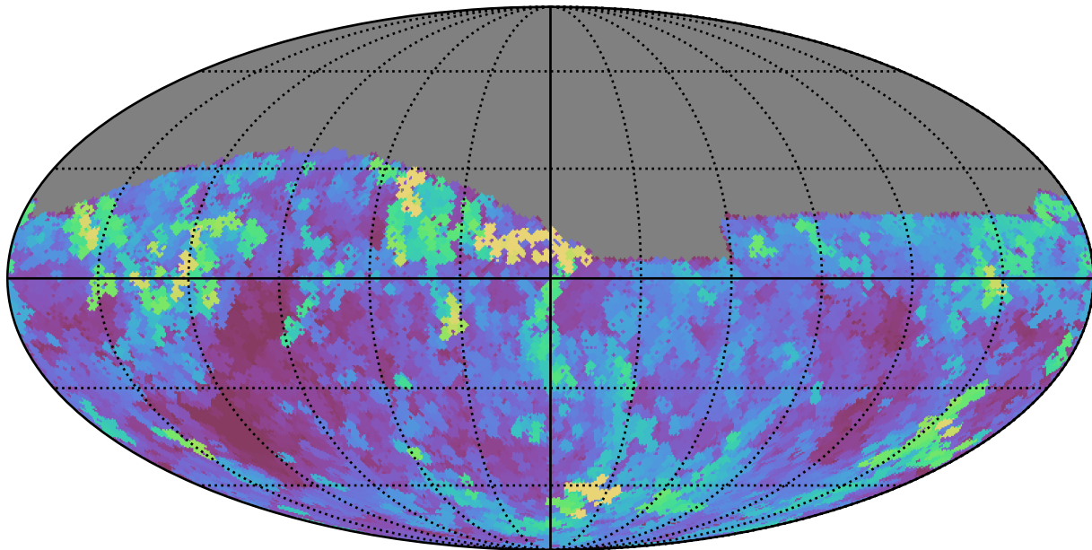
no_magell_roll_v3.4_10yrs Yr 1 i band: Max seeingEff
