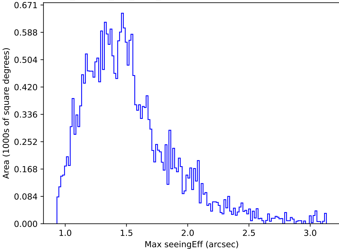
no_magell_roll_v3.4_10yrs Yr 1 g band: Max seeingEff
