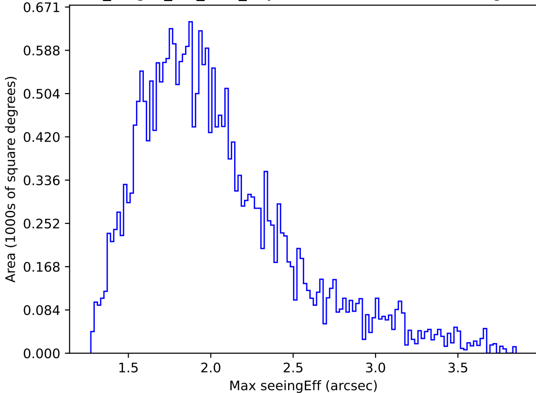
no_magell_roll_v3.4_10yrs Yr 1 all bands: Max seeingEff
