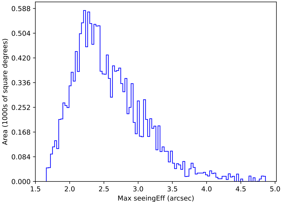
no_magell_roll_v3.4_10yrs WFD z band: Max seeingEff
