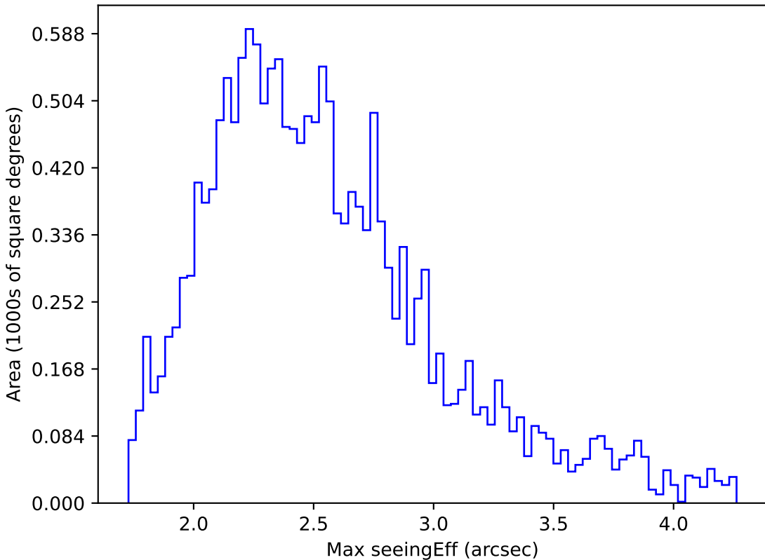
no_magell_roll_v3.4_10yrs WFD u band: Max seeingEff
