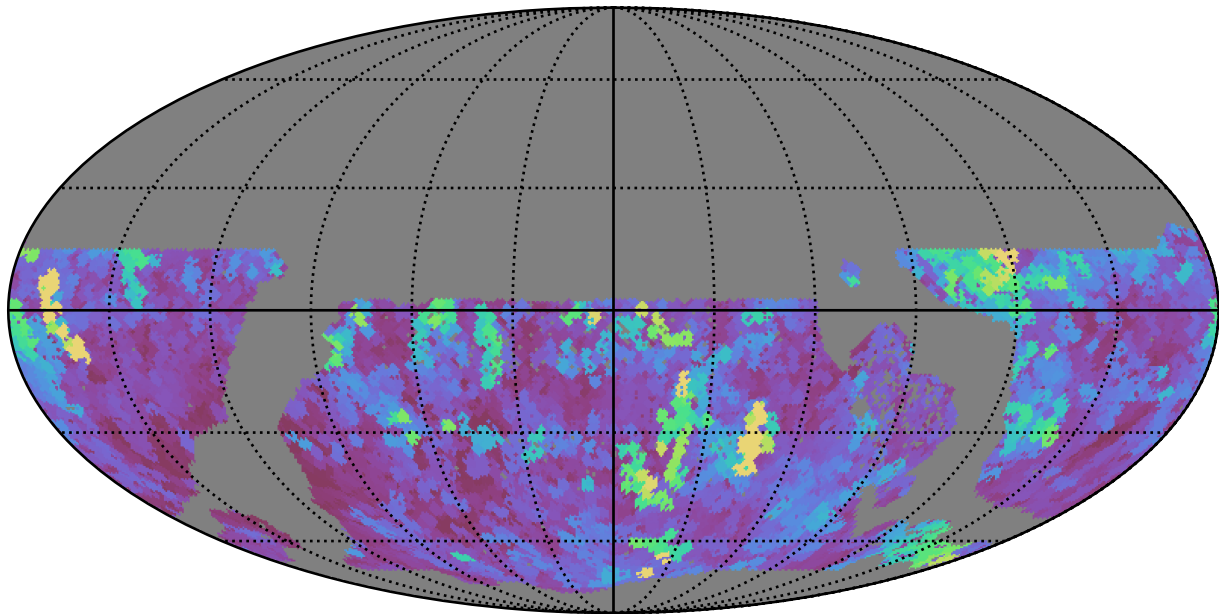
no_magell_roll_v3.4_10yrs WFD i band: Max seeingEff
