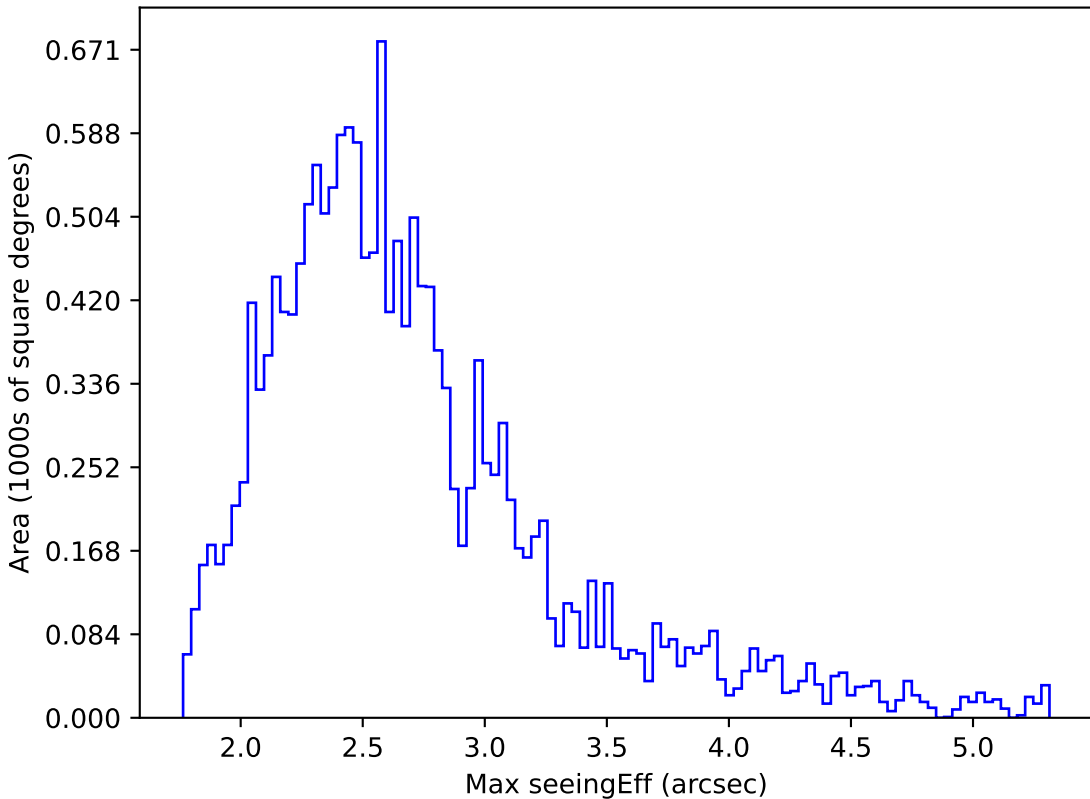
no_magell_roll_v3.4_10yrs WFD i band: Max seeingEff
